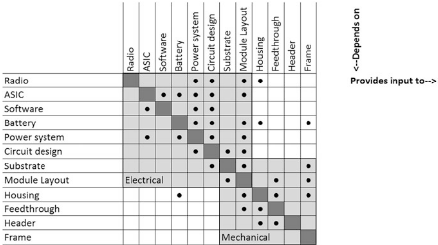
Fig. 11.2 Reorganized by engineering discipline, generic, simplified, component-based DSM for the components of a traditional pacemaker
