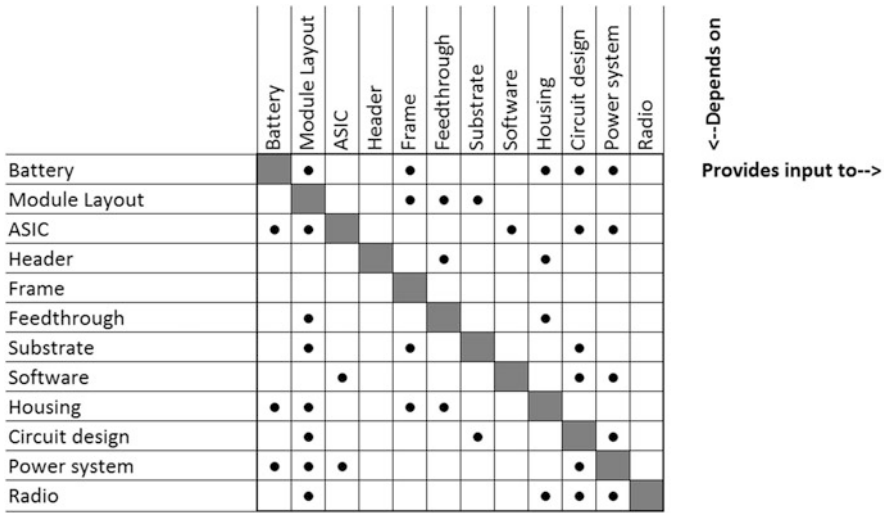
Fig. 11.1 Generic, simplified, component-based DSM for the components of a traditional pacemaker
